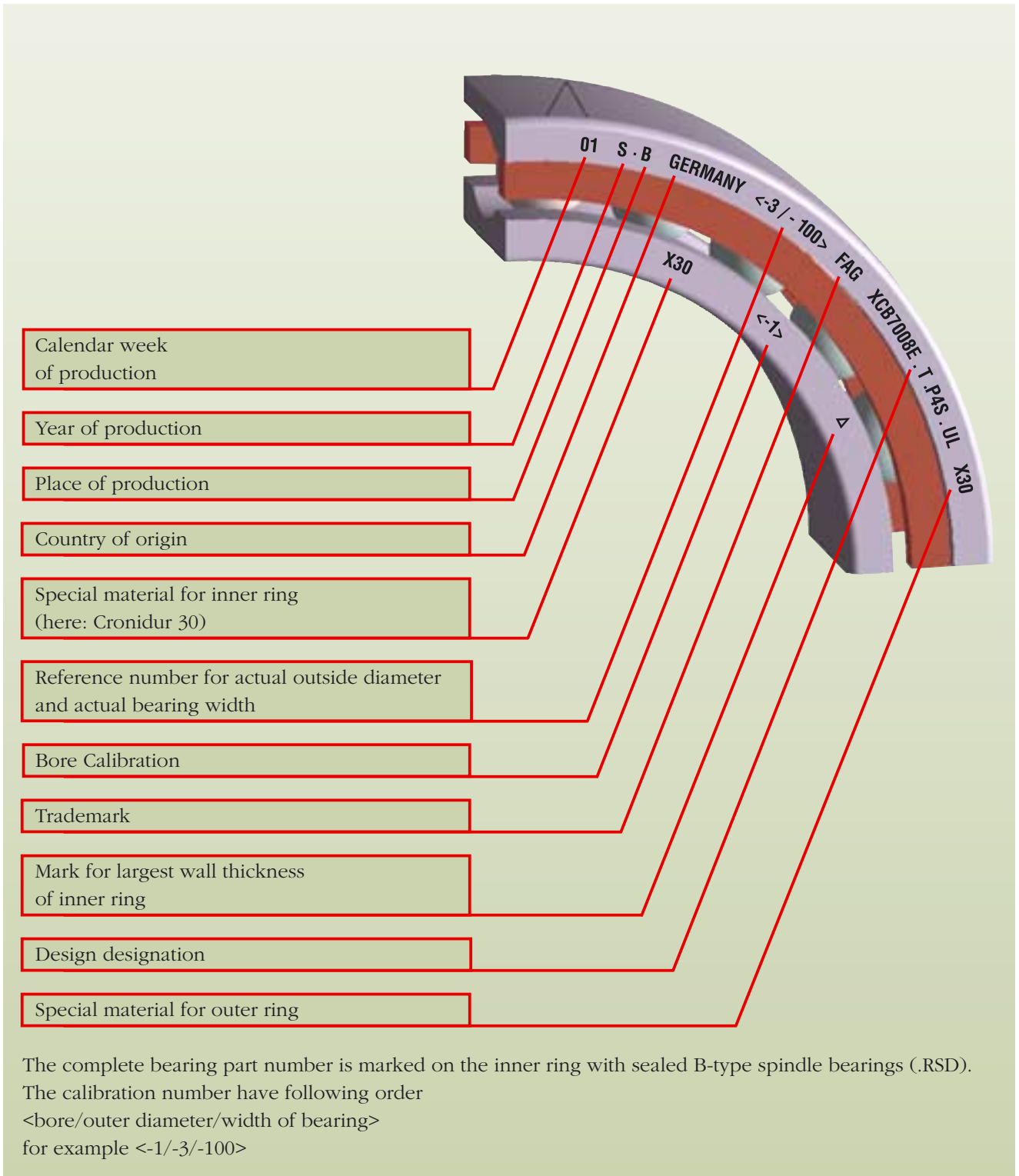
45: Designation details of FAG spindle bearings
